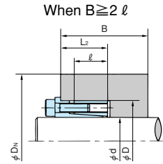
Installation Example(A) When installing to hubs with a guide portion, the hub configuration coefficient is as follows: K_3=0.8
