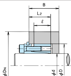
L_2 < B < 2L Hub Configuration Coefficient K_3=1.0
