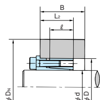
Installation Example(C)
