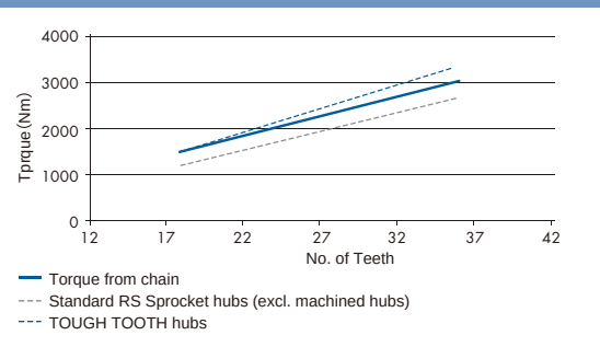
Comparison of Hub kW Ratings
