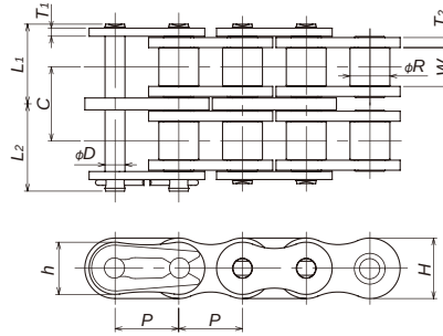
RS Double Strand Compatible LAMBDA Chain
