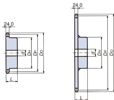
Mechanically machined 1B type
