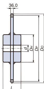
Welded construction 1C type
