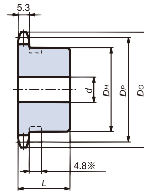
(Machined specifications) 1B Type
