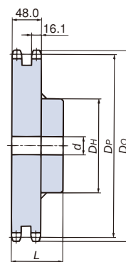
(Machined specifications) 2B Type
