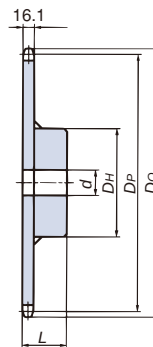
(Machined specifications) 1B Type
