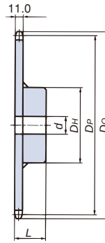
(Welded specifications)
