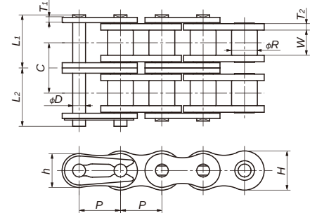
Conventional Double Strand LAMBDA Chain
