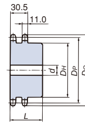
(Machined specifications) 2B type
