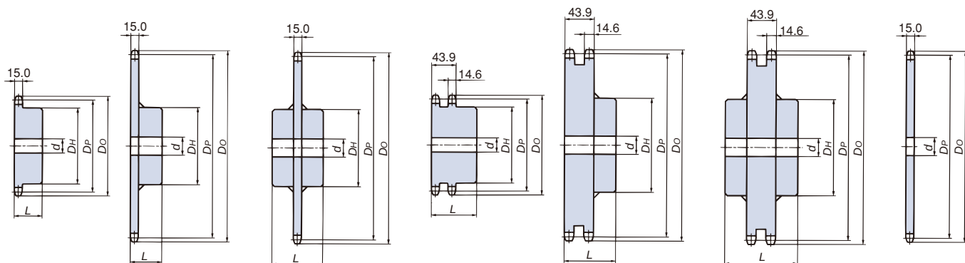
Mechanically machined Welded construction Welded construction Mechanically machined Welded construction Welded construction 1A type 1B type 1C type 2B type 2C type
